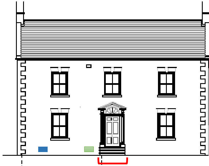
Front (West) elevation
