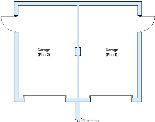
Twin Garage Plan Plots 1 & 2
