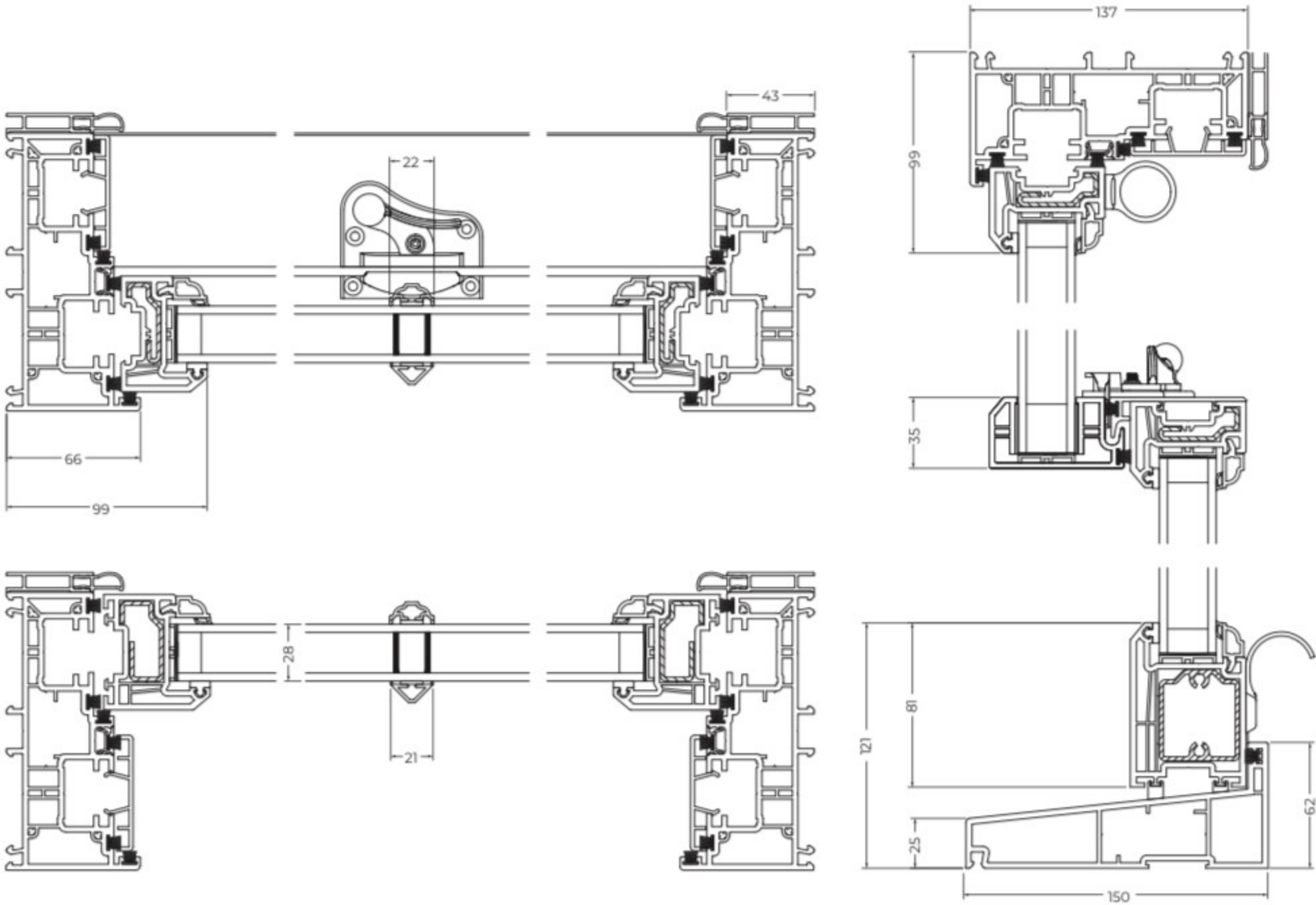
Flush standard cill option
