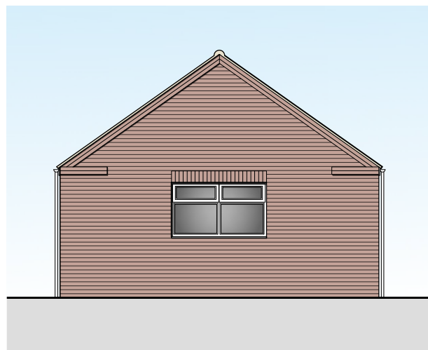
Existing Side (W) Elevation Scale 1:100
