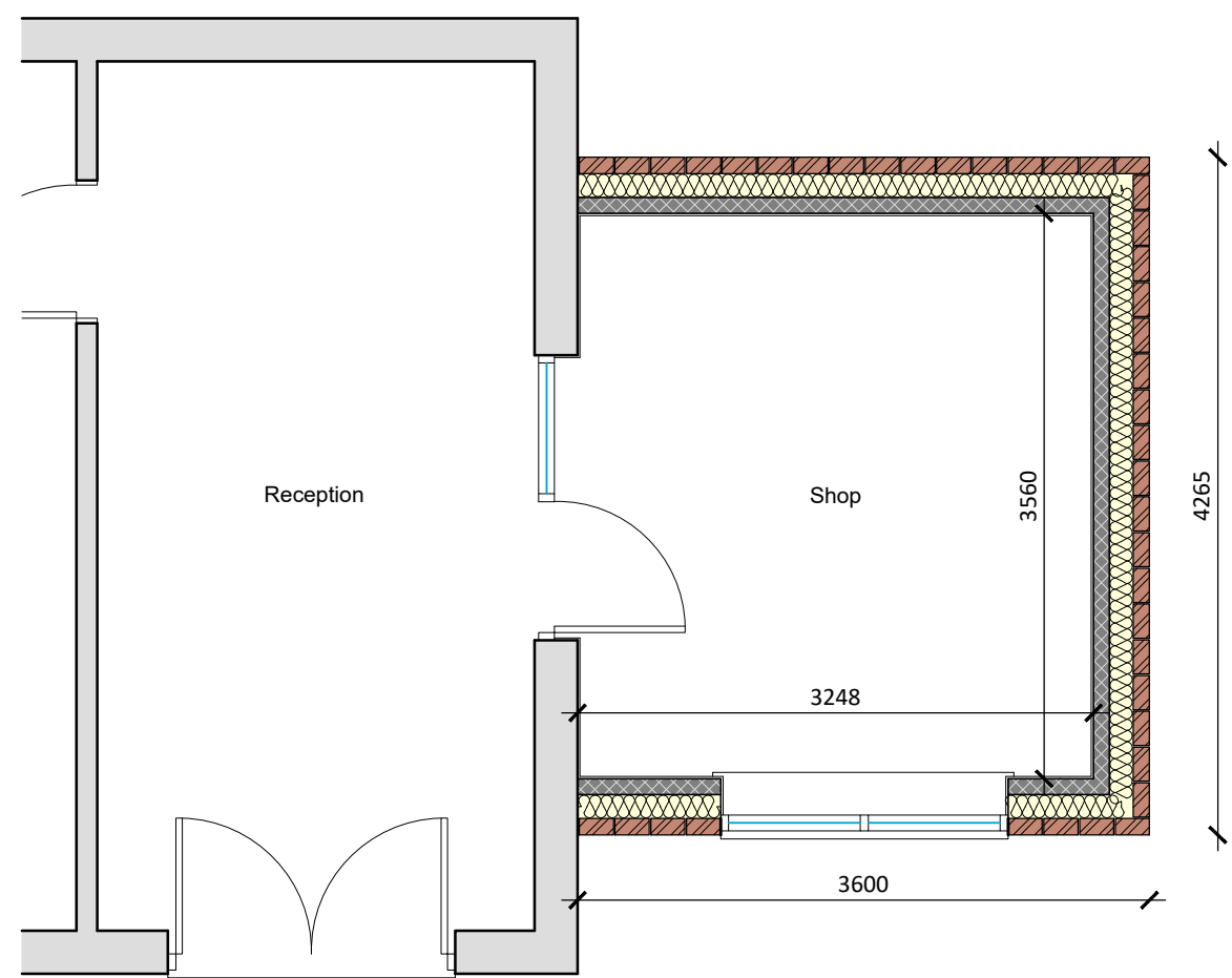
Proposed Part Floor Plan Scale 1:50
