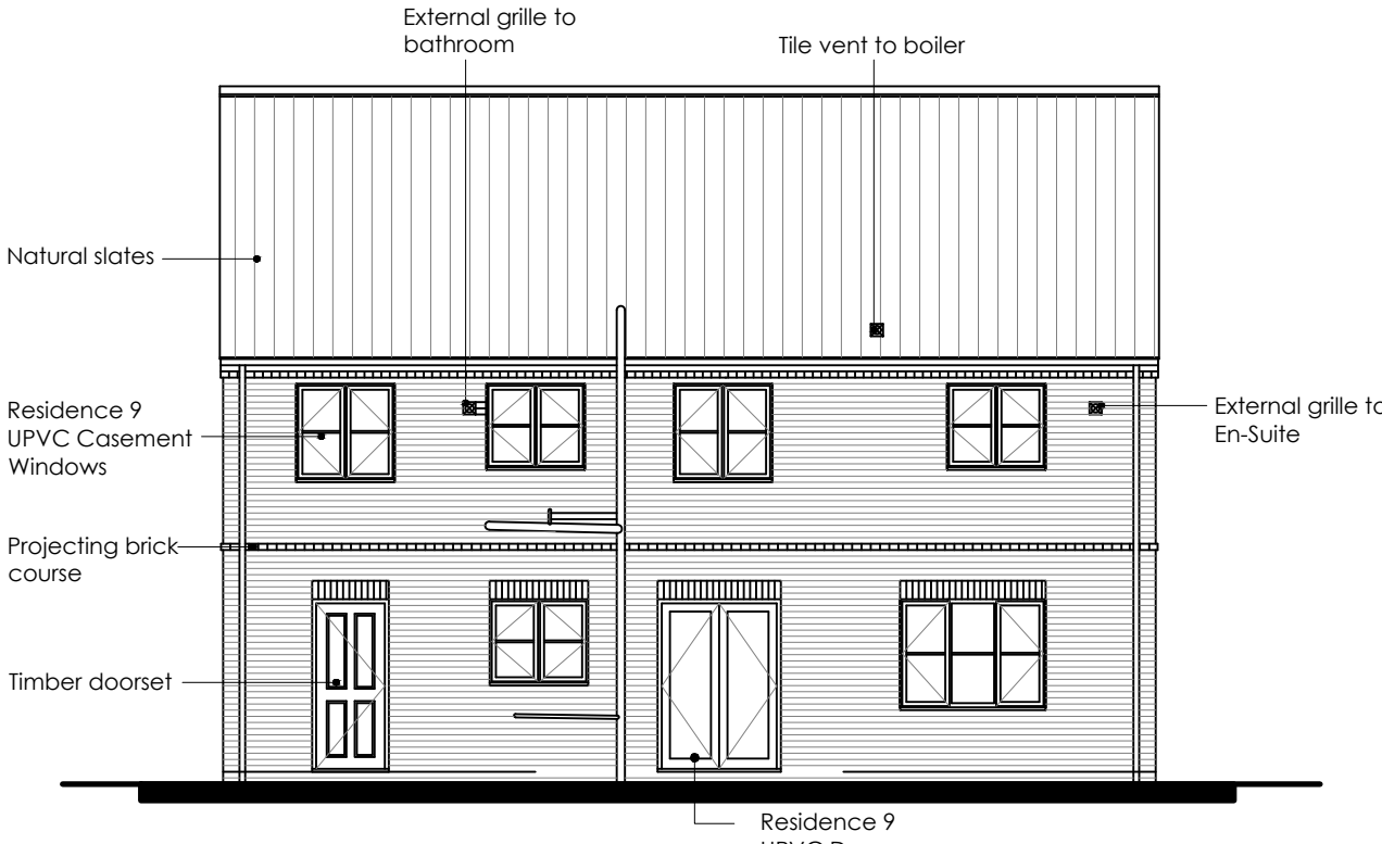
REAR ELEVATION
