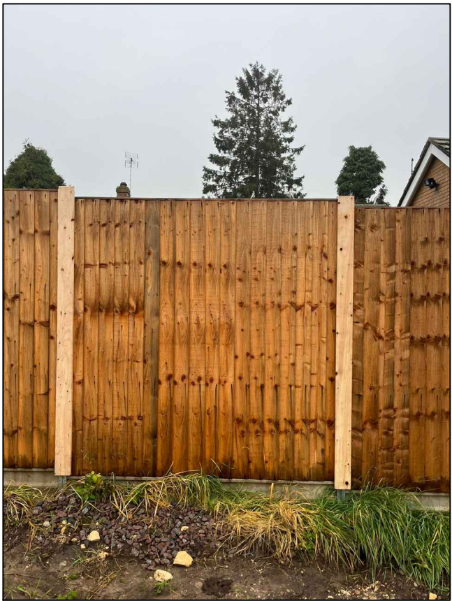
DURAPOST SUPPORT INSTALLATION AFTER CLADDING APPLIED N.T.S.
