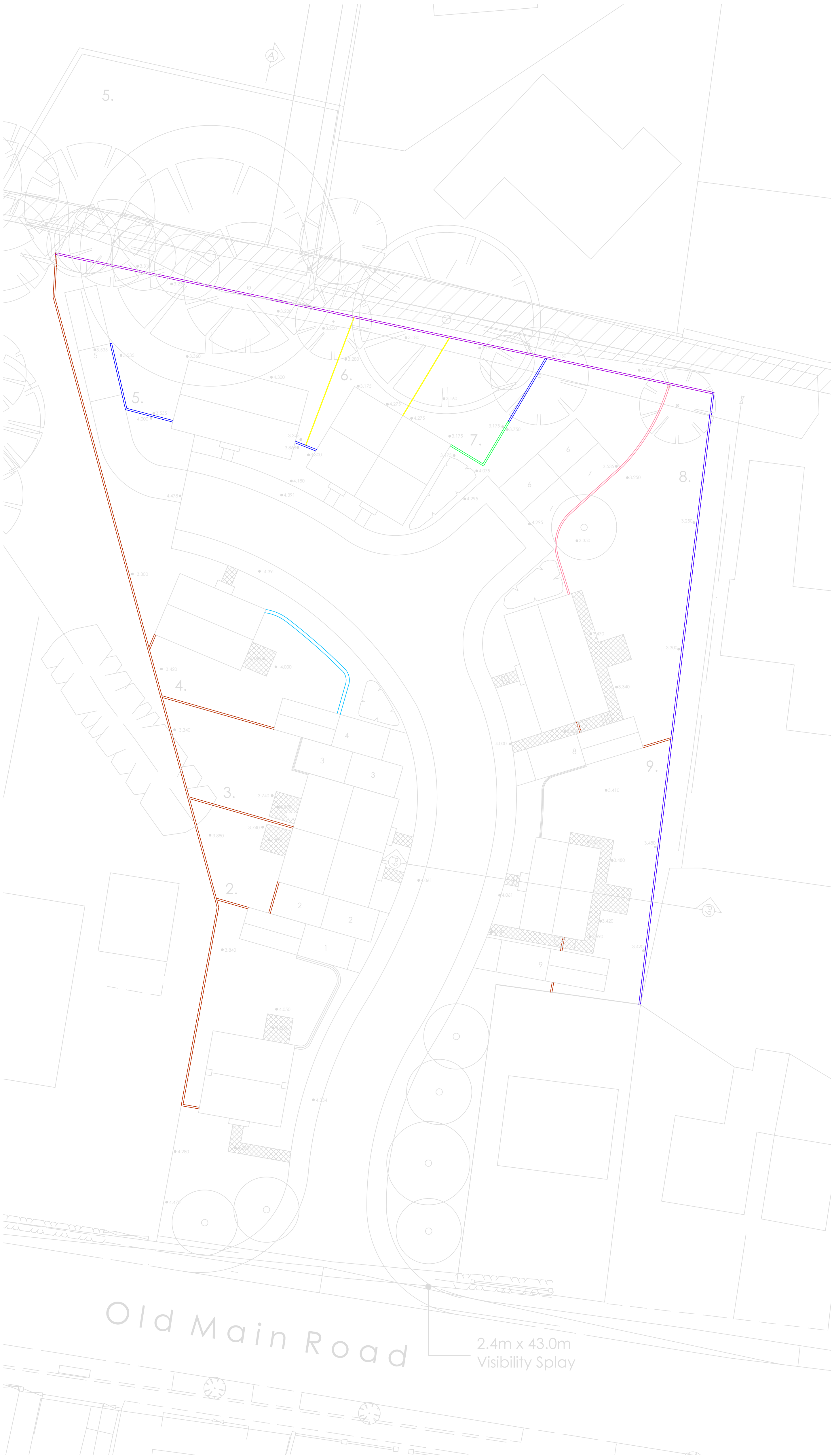
BOUNDARY TREATMENT PLAN
