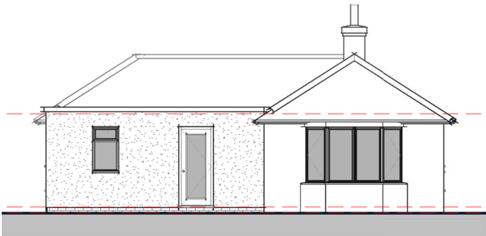
Elevation 03 - Rear 1 : 100
