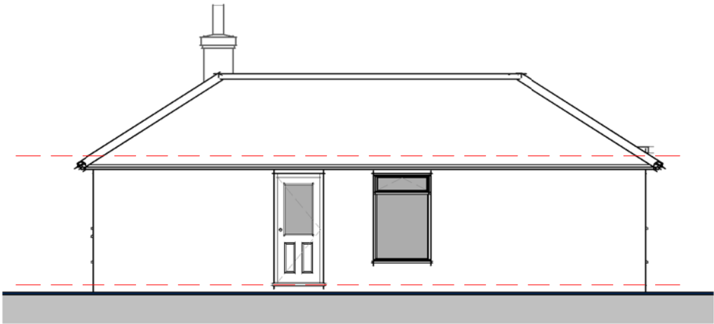
Elevation 01 - Front 1 : 100
