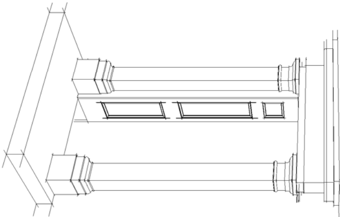
3D View Door Surround
