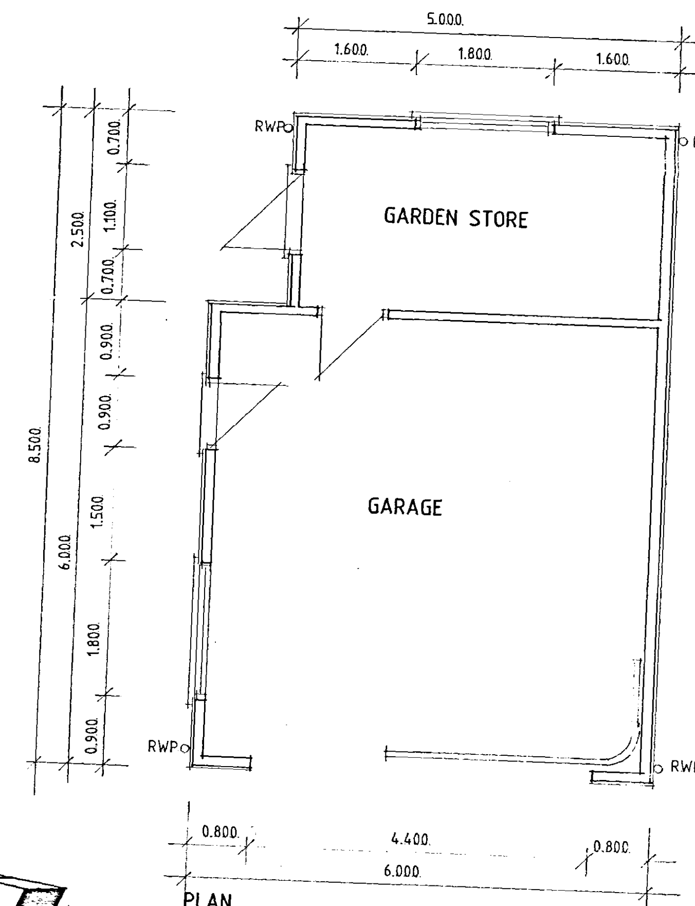
PROPOSED GARAGE/GARDEN SHED
