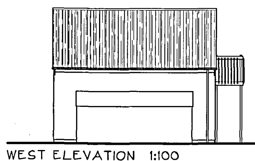
WEST ELEVATION 1:100
