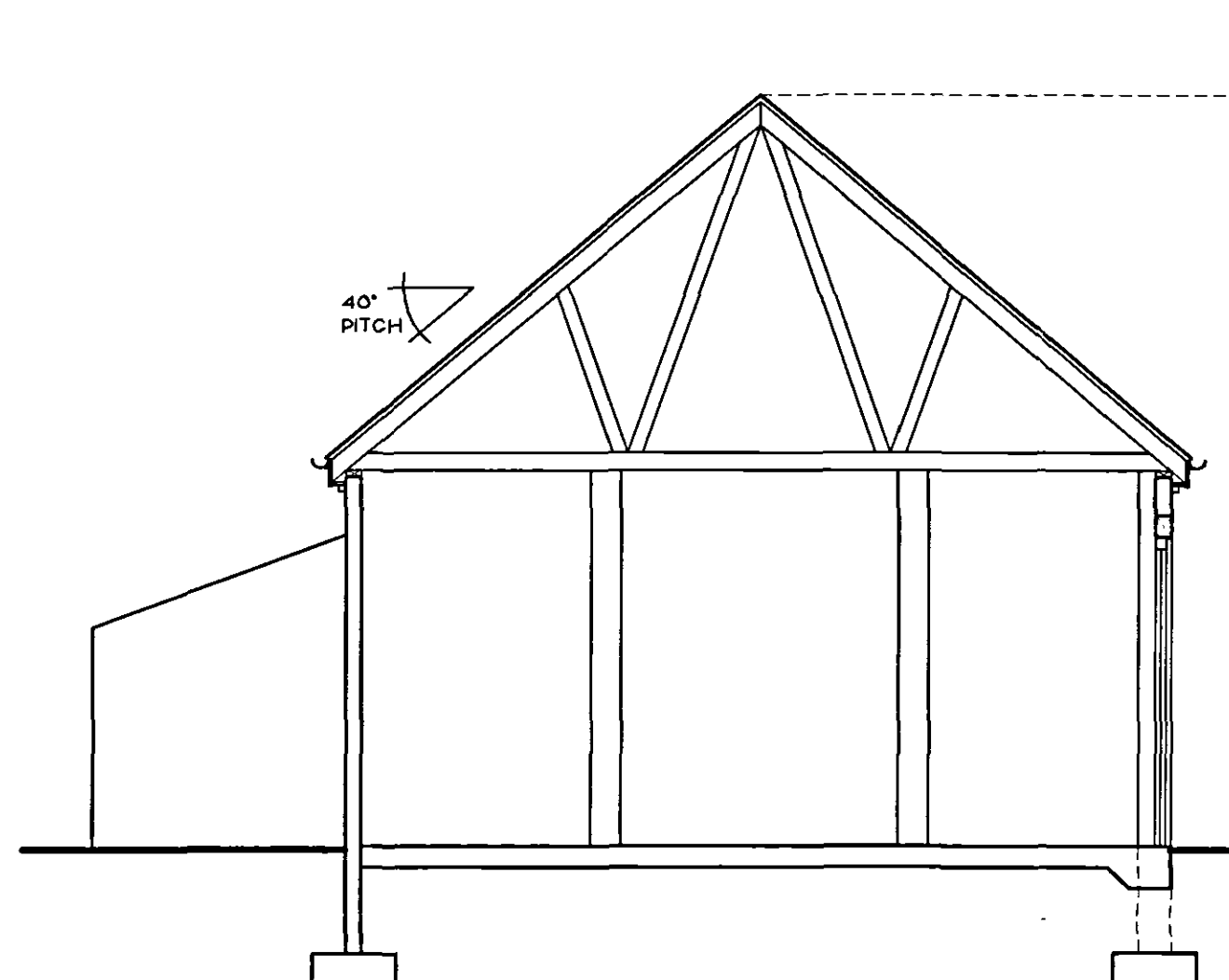
EXISTING SECTION 1:50
