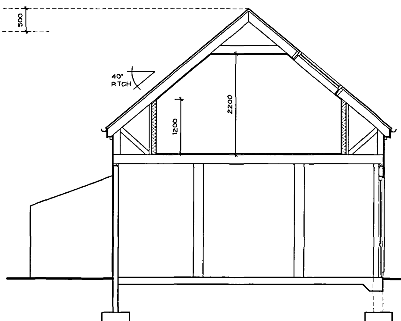
PROPOSED SECTION 1:50
