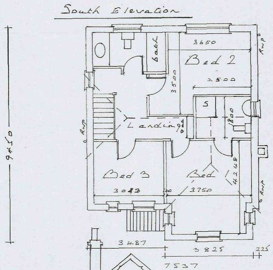
Side South Elevation
