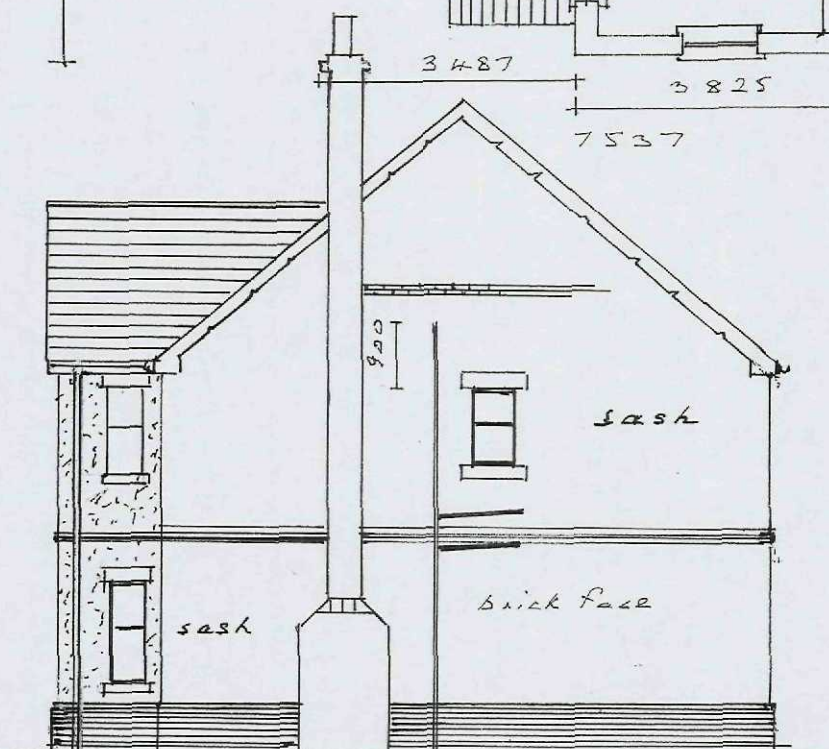
Side North Elevation
