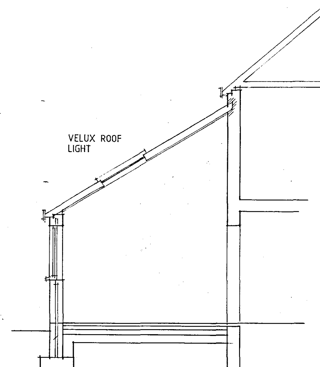
SECTION
