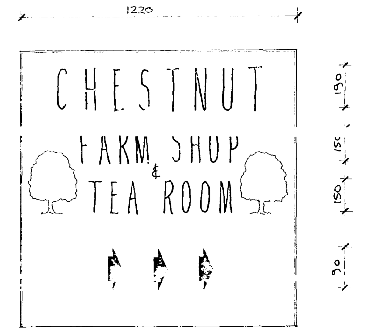
Sign No. 4. marked on wall of building bottom of sign to be 1.40m above g.l.
