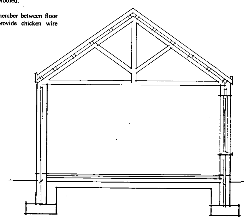
SECTION THRO' TEA ROOM
