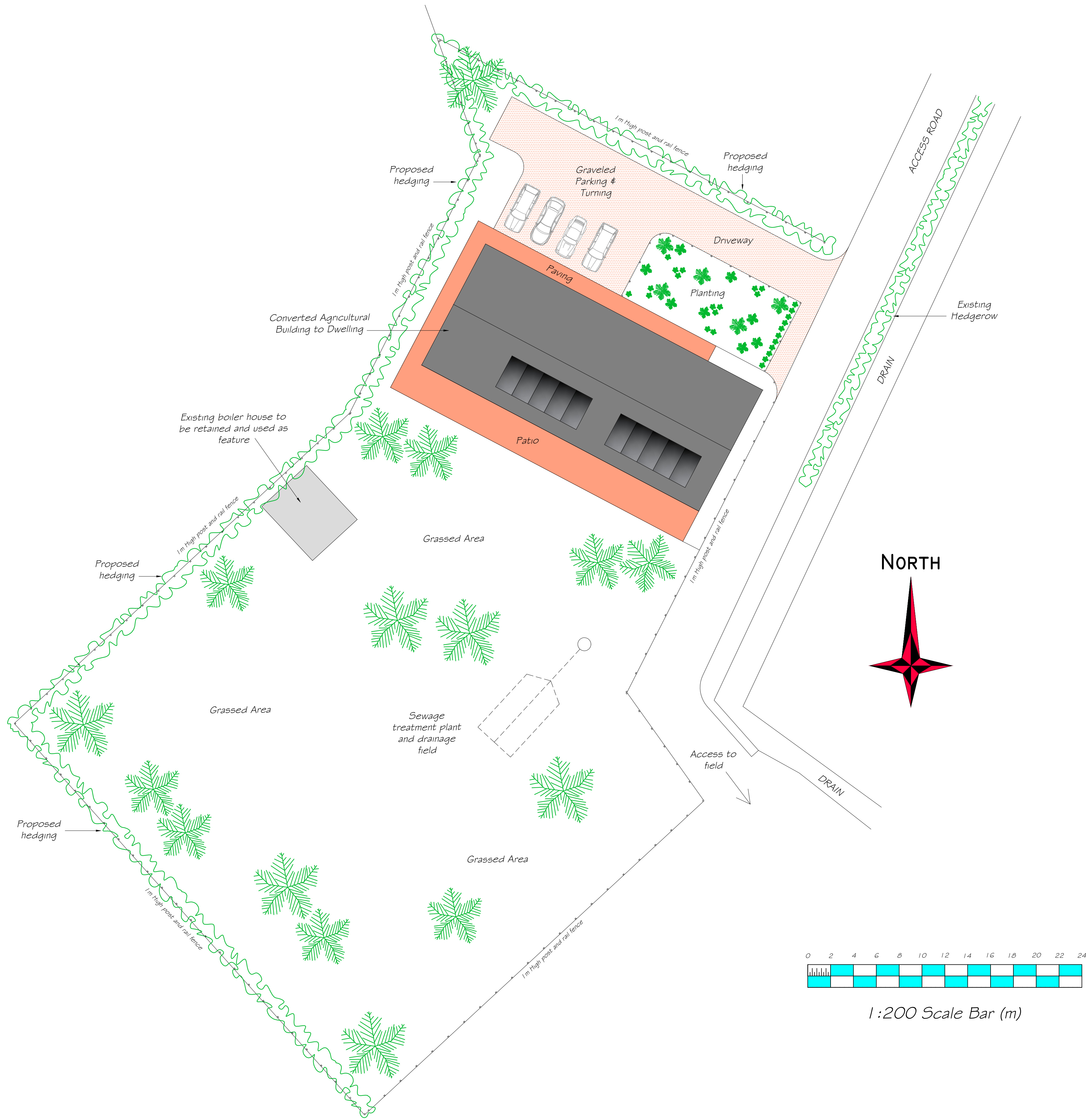
PROPOSED BLOCK PLAN 1:200
