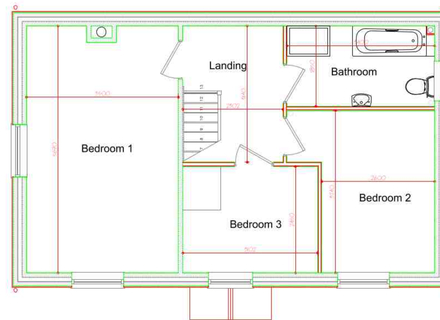
PROPOSED FIRST FLOOR 1:50
