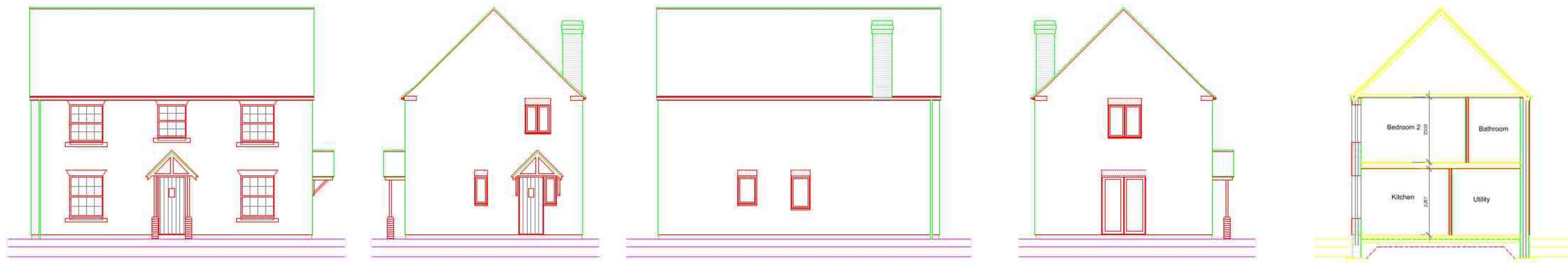
PROPOSED ELEVATIONS 1:100
