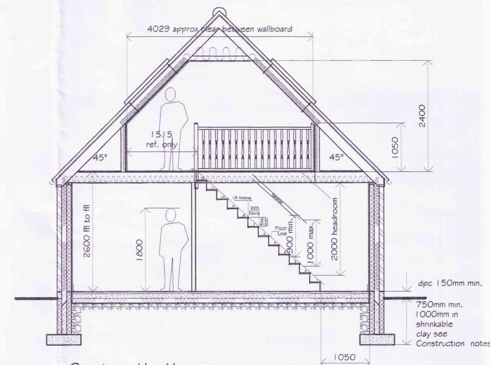
Section X - X Scale 1/50
