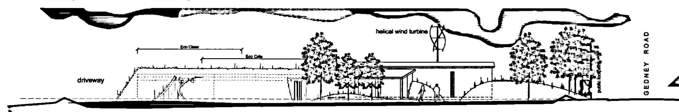
Driveway (North - West) Elevation 1:200
