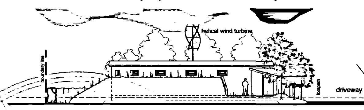
(North - East) Elevation 1:200
