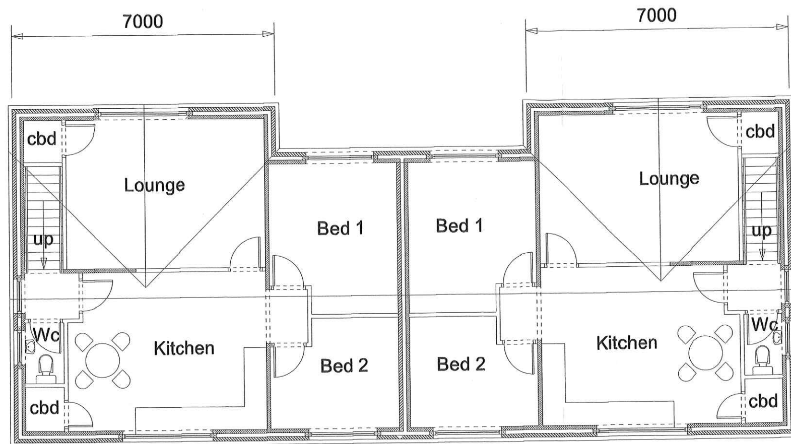
First Floor
