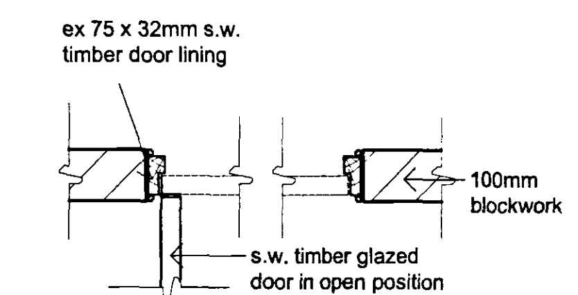
# Detail W (Internal Door Jambs) 1:20
