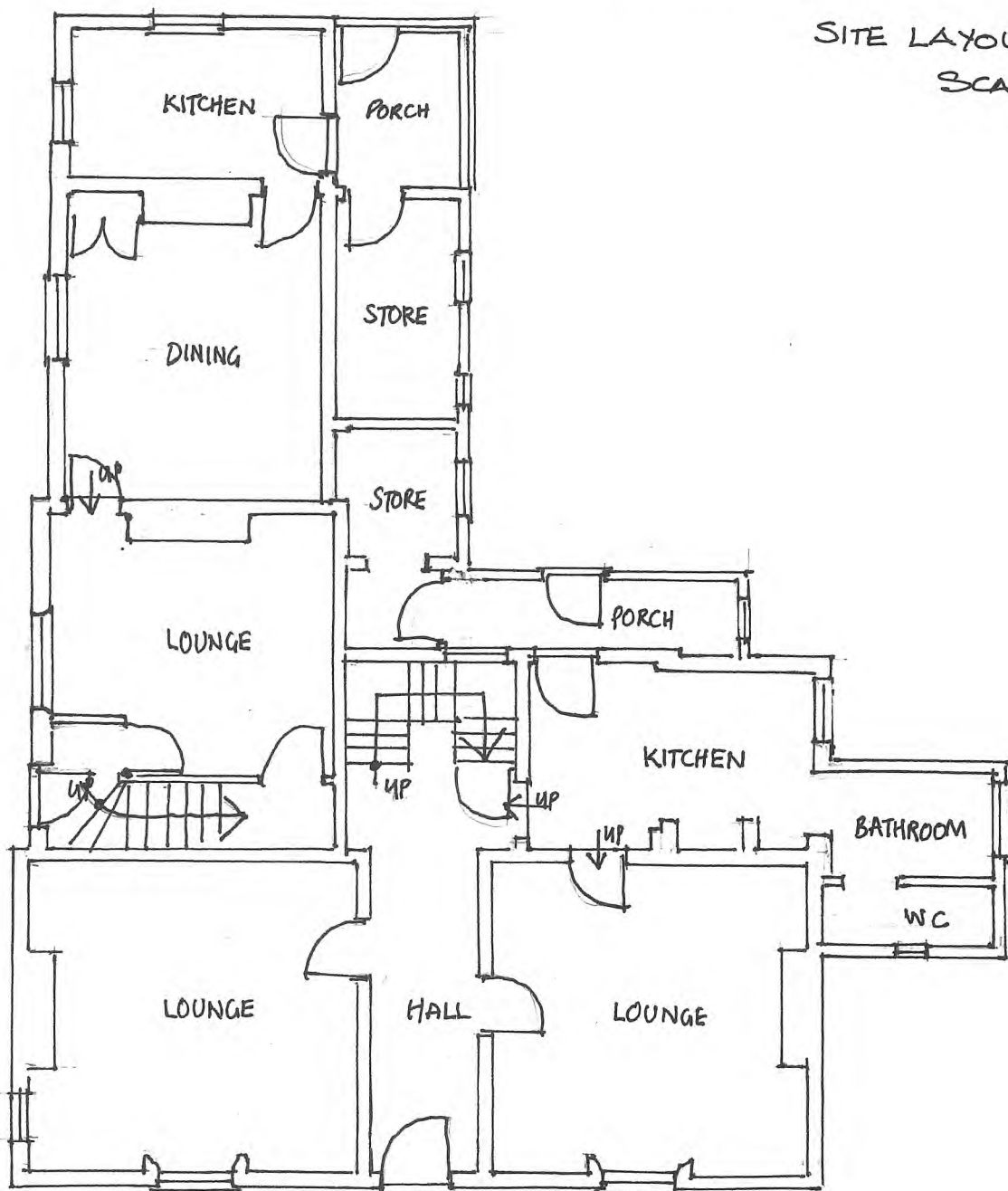
PLAN LAYOUT EXISTING SCALE 1:100
