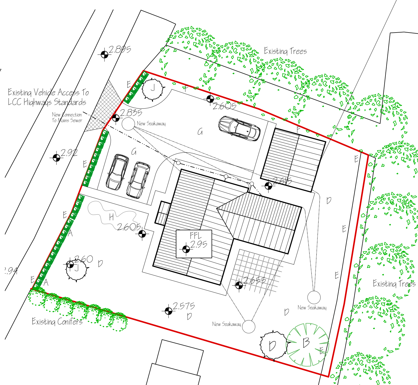
SITE PLAN - PROPOSED 1:250
