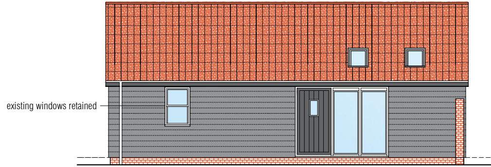
east elevation
