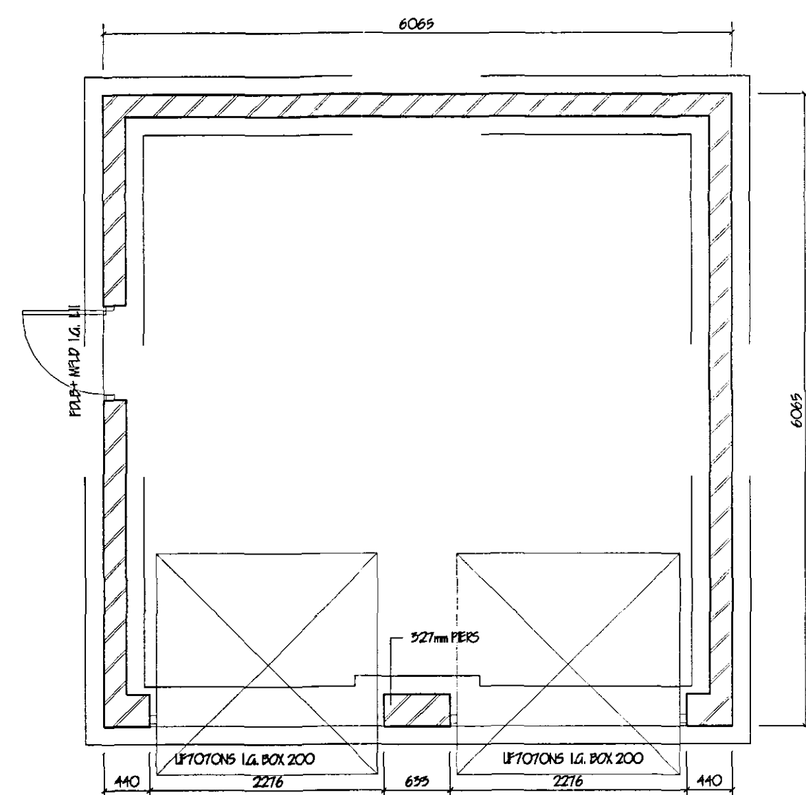
FLOOR PLAN
