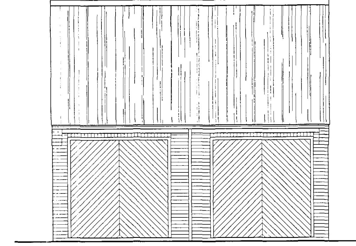
FRONT ELEVATION
