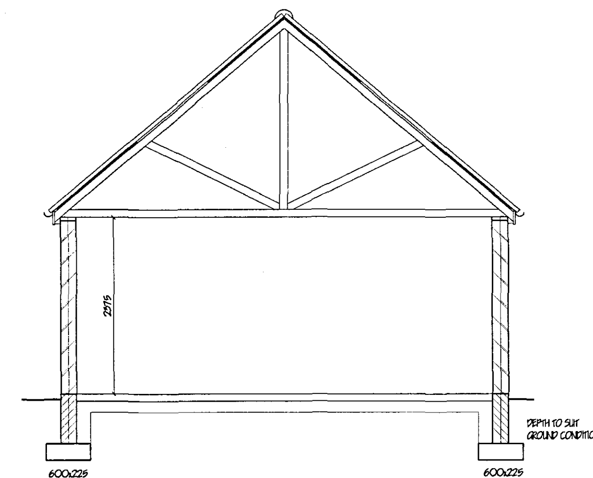
SECTION
