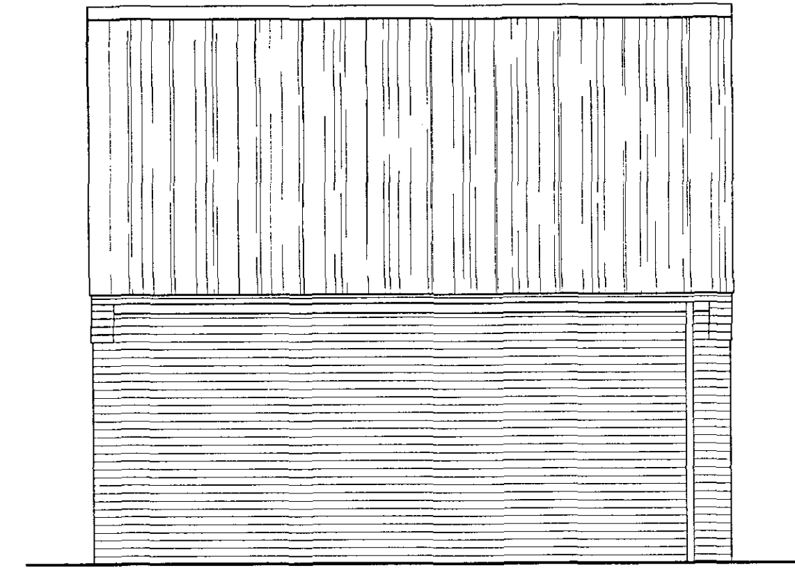
REAR ELEVATION
