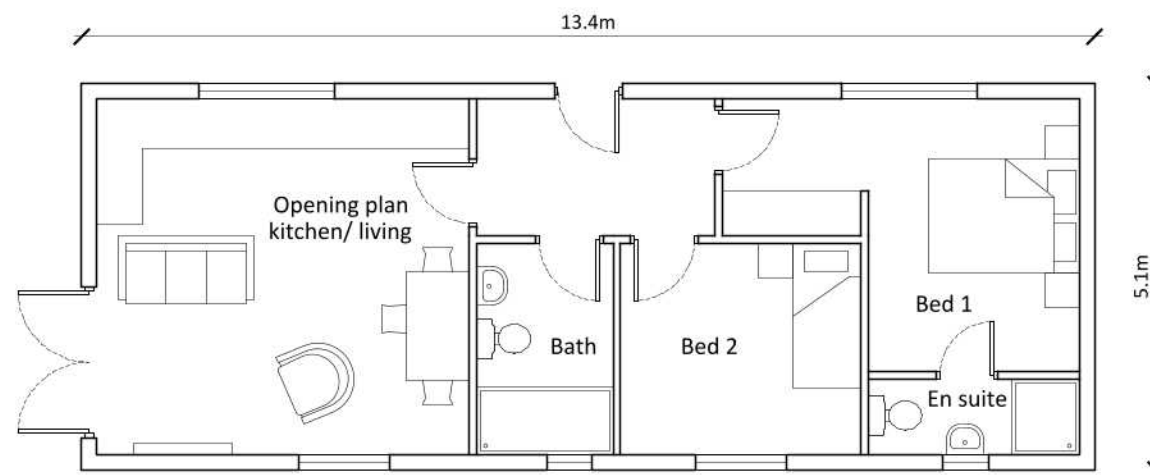
Floor Plan
