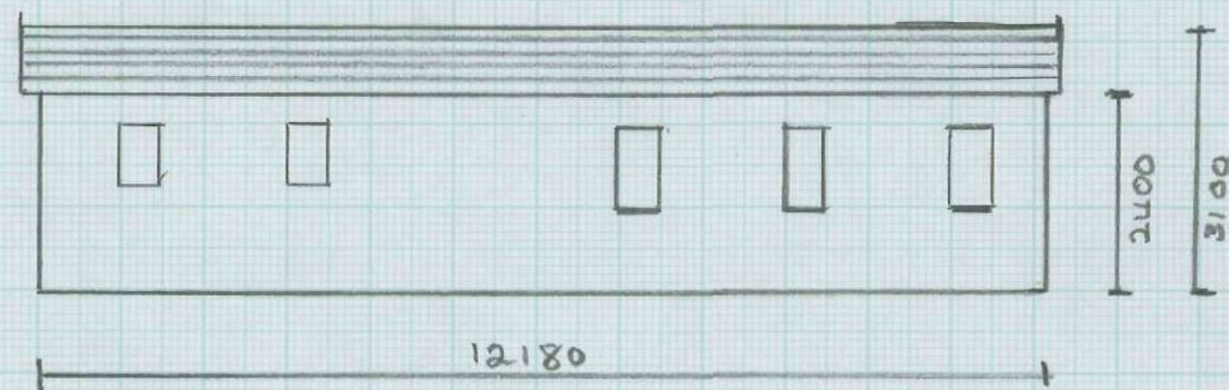
South Elevation
