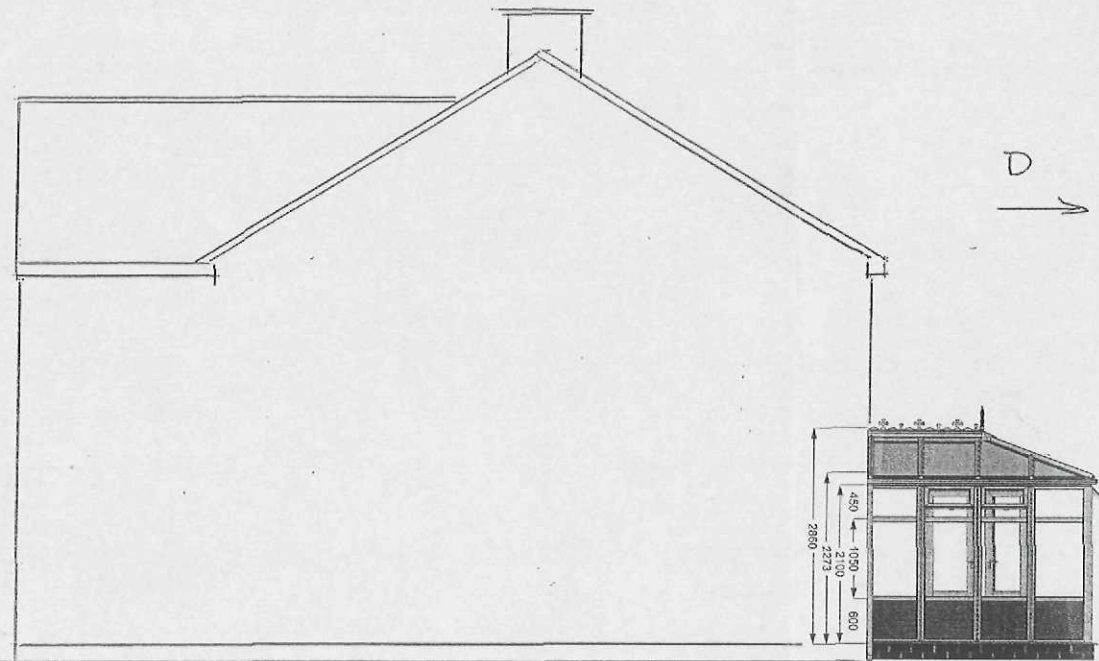
Proposed RIGHT HAND ELEVATION "B"
