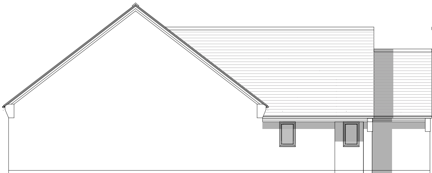
SIDE ELEVATION 2
