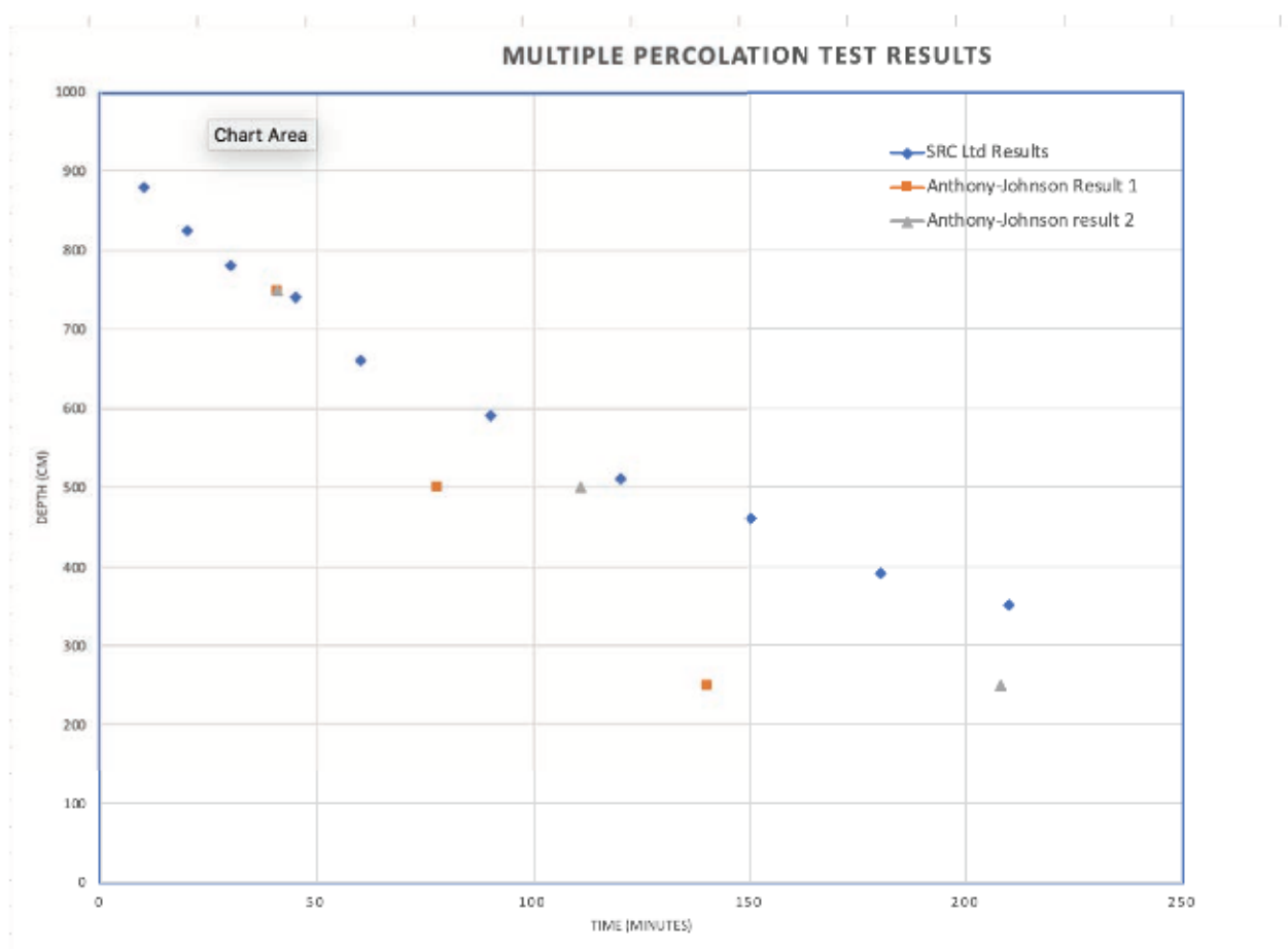
Image 10.0: Percolation test results
