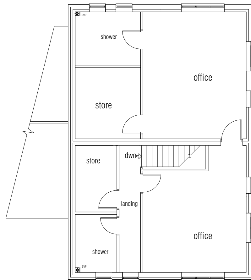
First Floor as Existing
