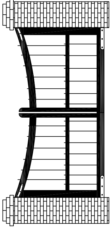
Gate Elevation Scale 1:50
