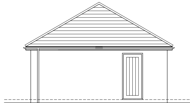
side elevation ( towards bungalow )
