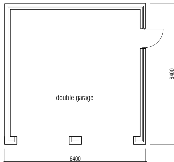
Floor Layout
