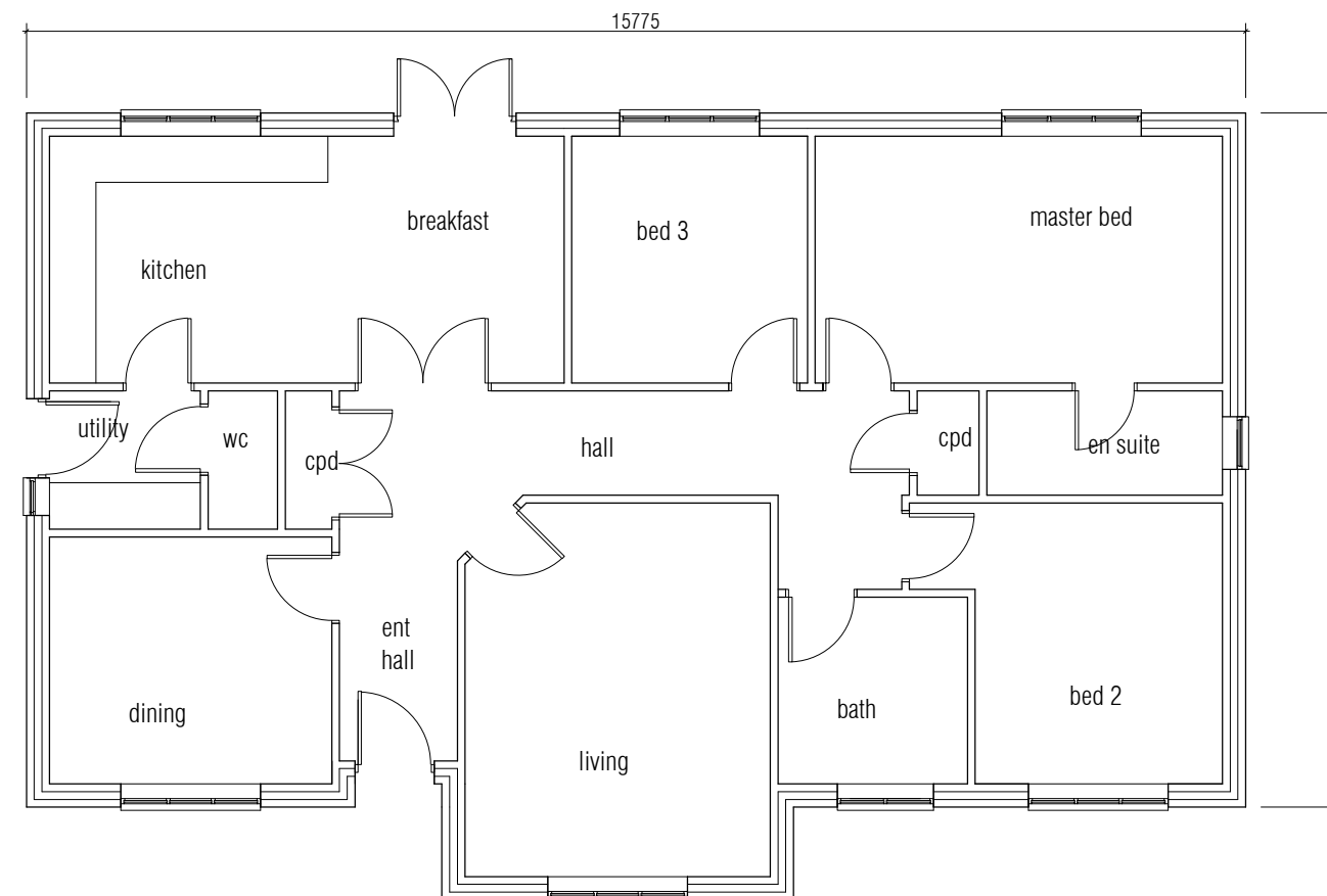
Floor Layout 1:100 scale
