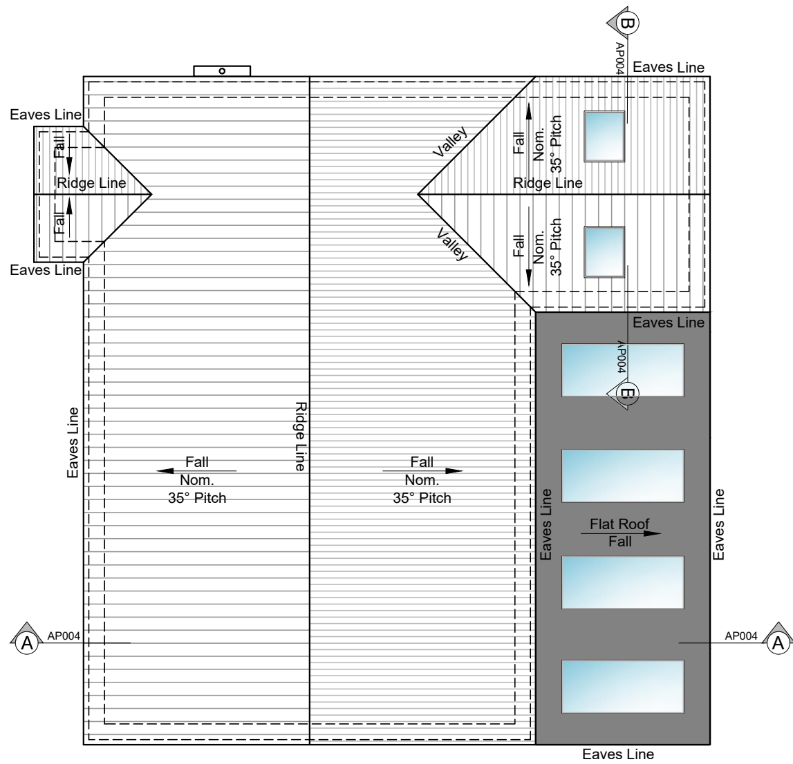
Roof Plan
