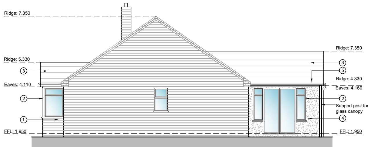
South Elevation
