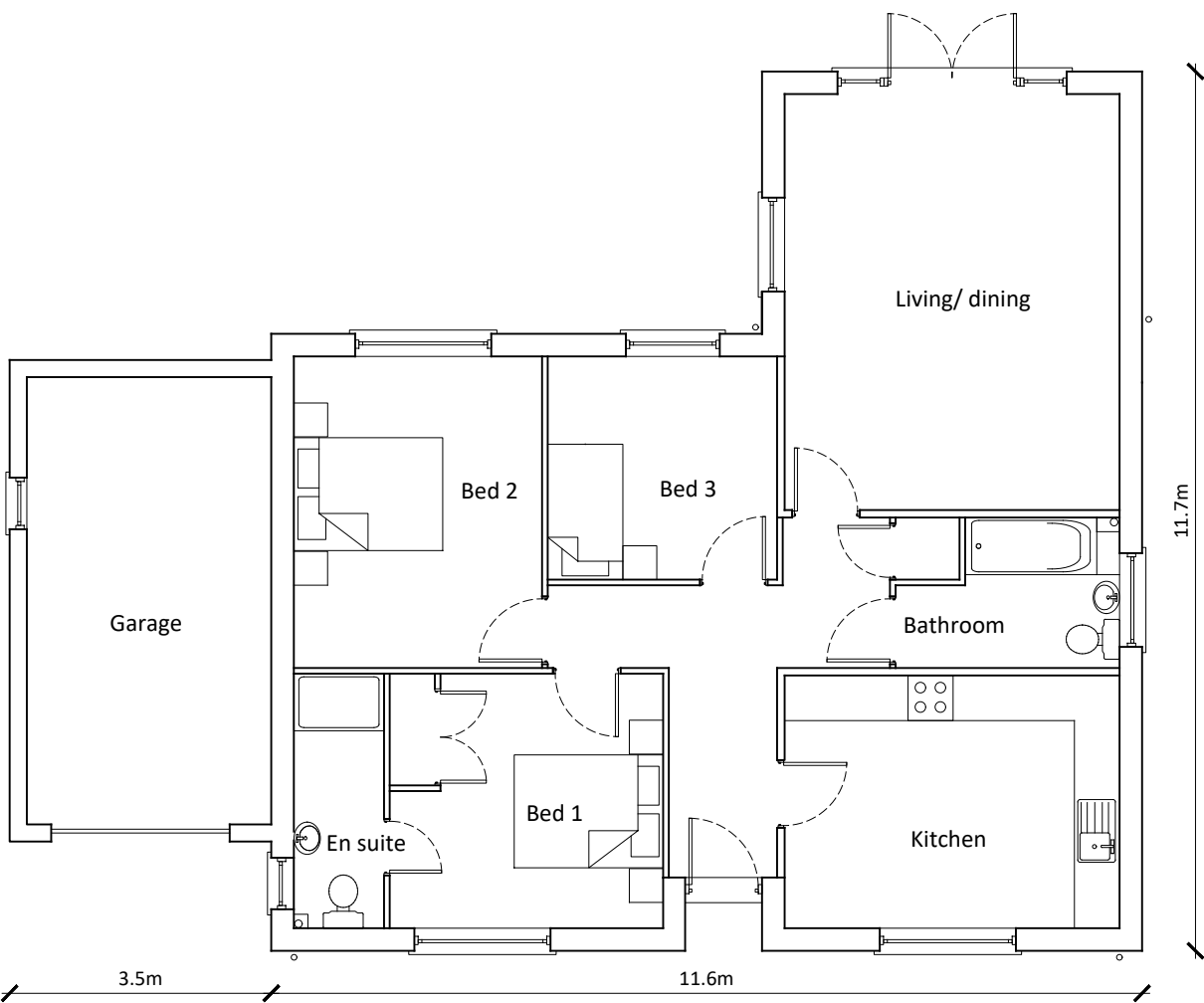
Floor Plan
