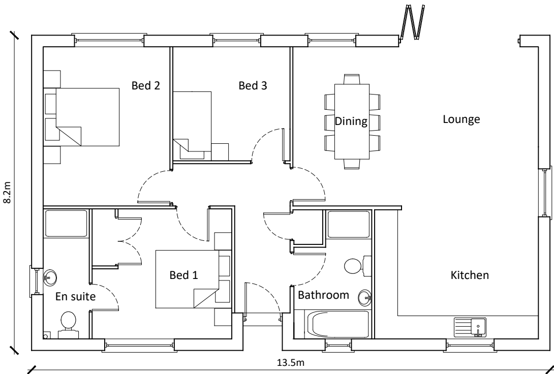
Floor Plan
