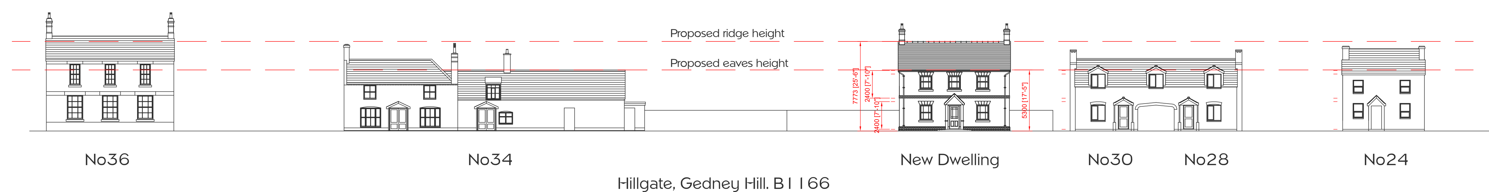
Proposed Street Scene Elevation Elevations 1:200 @ A1
