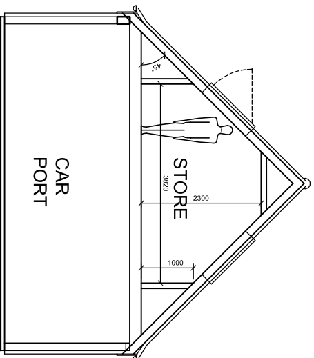
Preliminary Section
