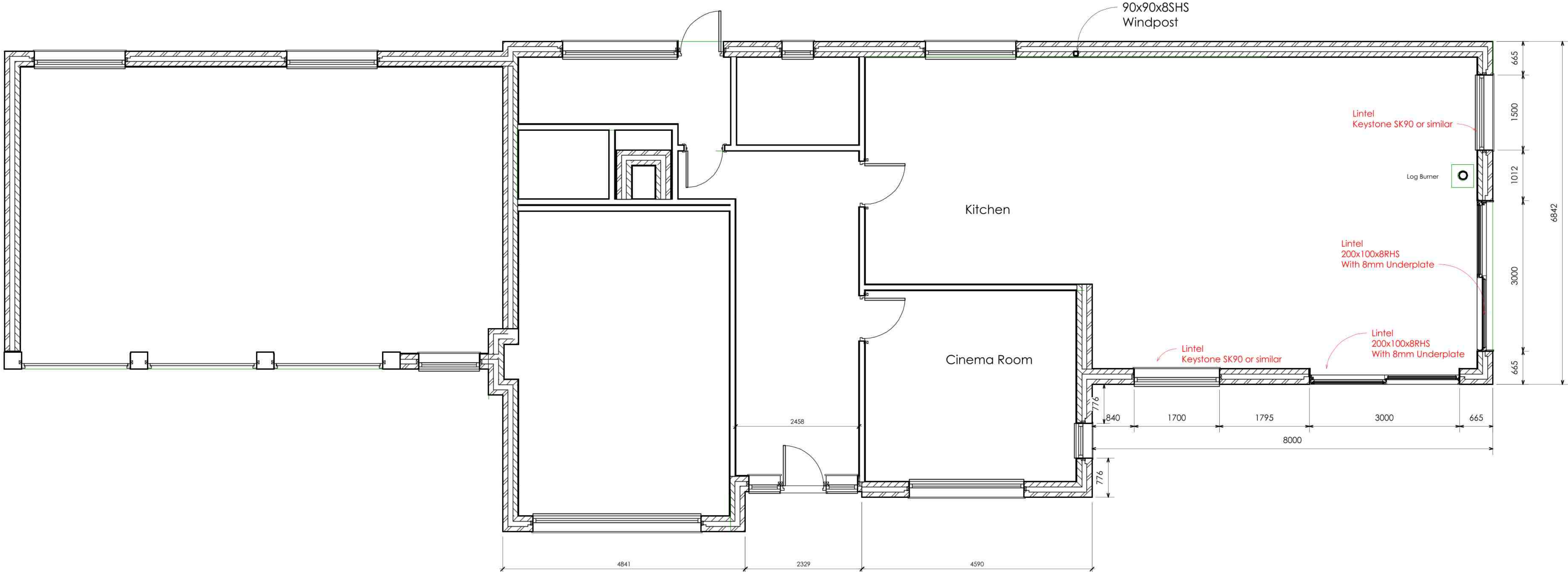
1 Ground 1 : 50
