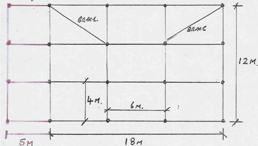
ROOF PLAN.
