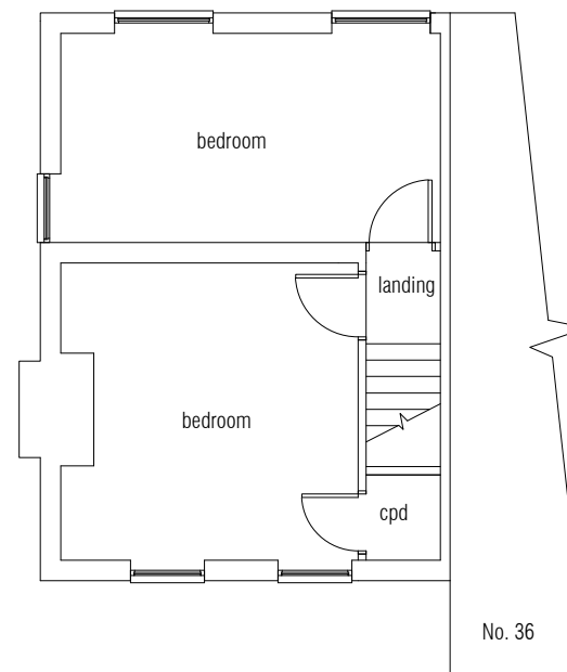
first floor - existing dwelling
