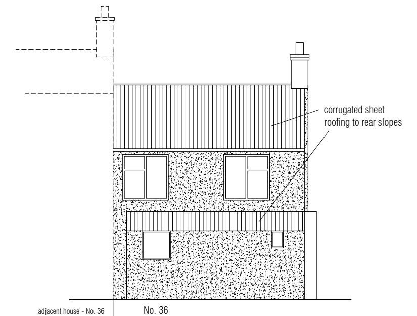
rear elevation
