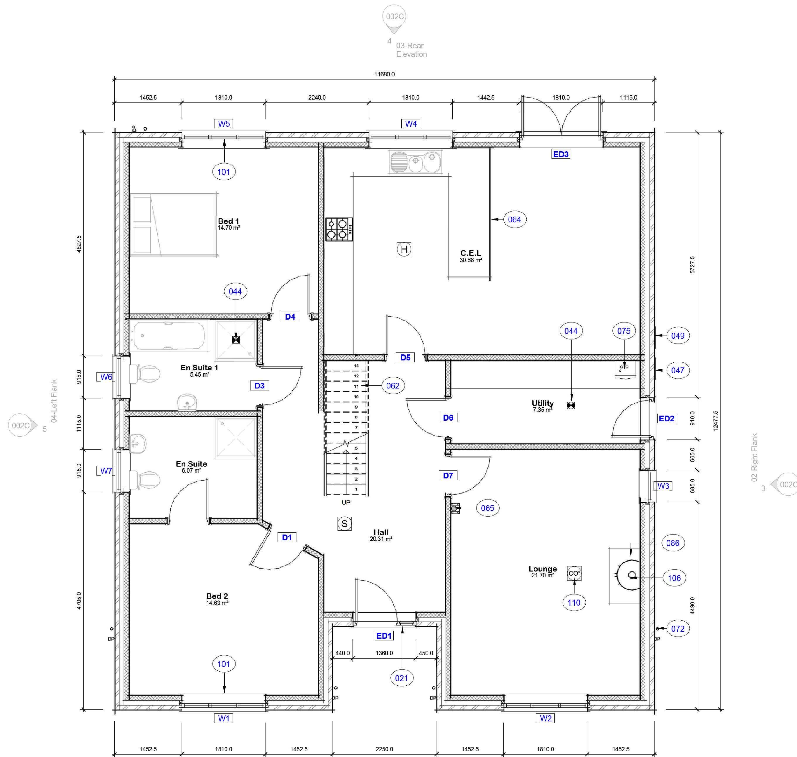
01-Ground Floor 1 : 50
