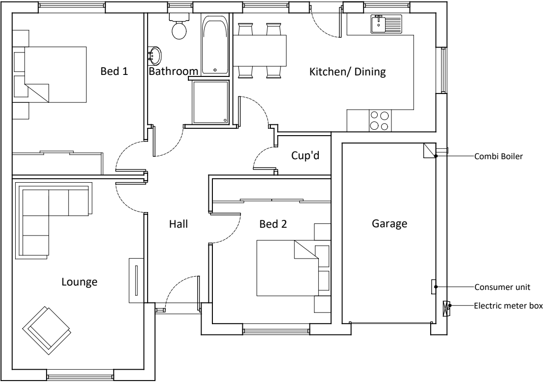
Floor Plan
