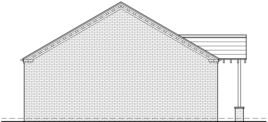
Side Elevation
