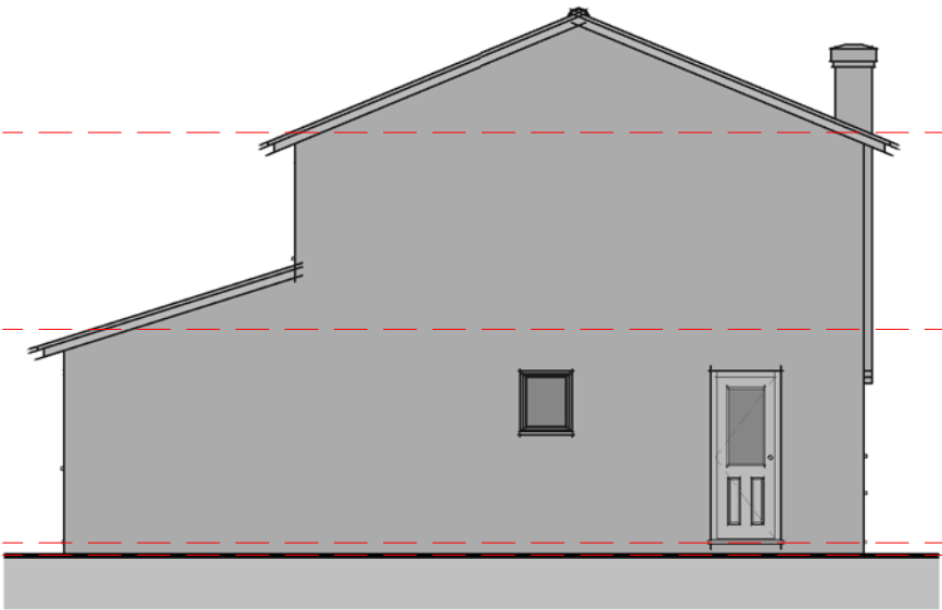
Elevation 02 – Right 1 : 100
