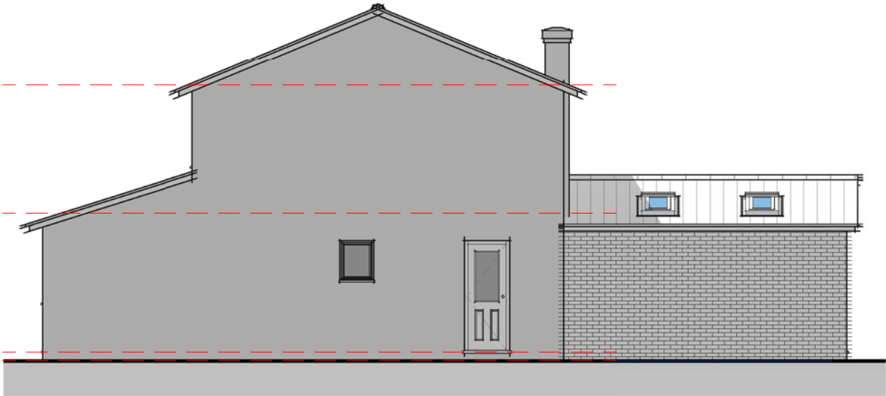
Elevation 02 – Right 1 : 100
