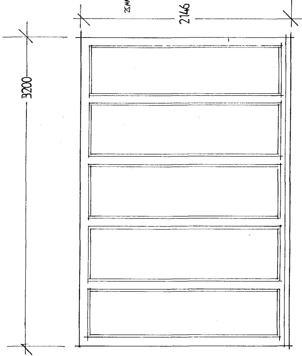
ELEVATION 1.20
