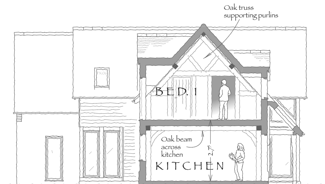
SECTION
