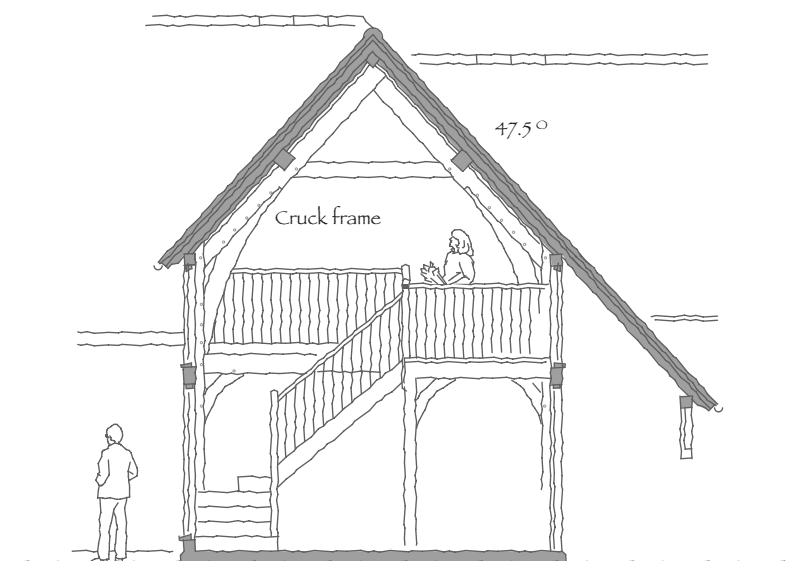
SECTION THRO' HALL
